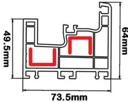
Mono rail frame profile
