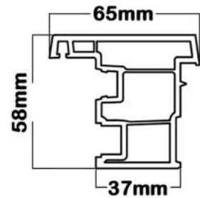
Lap joint profile
