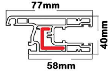
Sliding window sash profile
