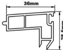
Mono rail cover profile
