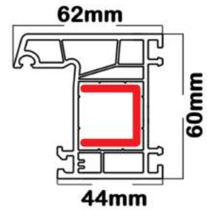
Frame profile
