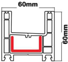
2 track sliding frame profile
