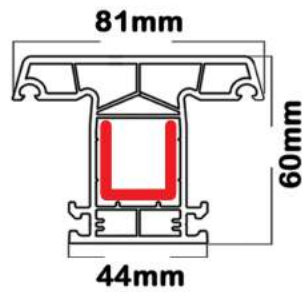
Mullion profile
