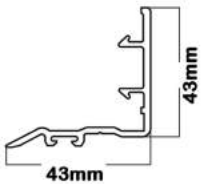
Sliding window interlock
