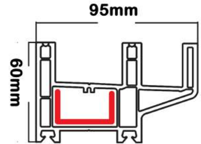
3 track sliding frame profile
