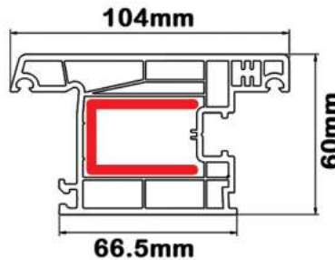
Door sash outward open profile
